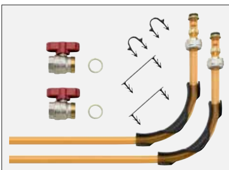
Example: Connection set of components for heating pipes with a diameter of 16 mm
